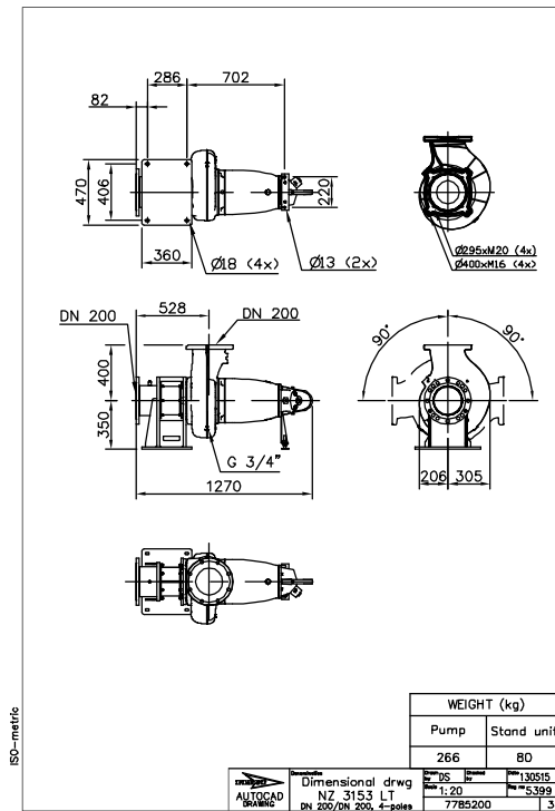
Figure 19: LT, Z-installation
