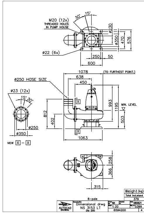
Figure 16: LT, S-installation
