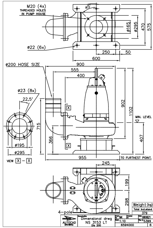
Figure 15: LT, S-installation
