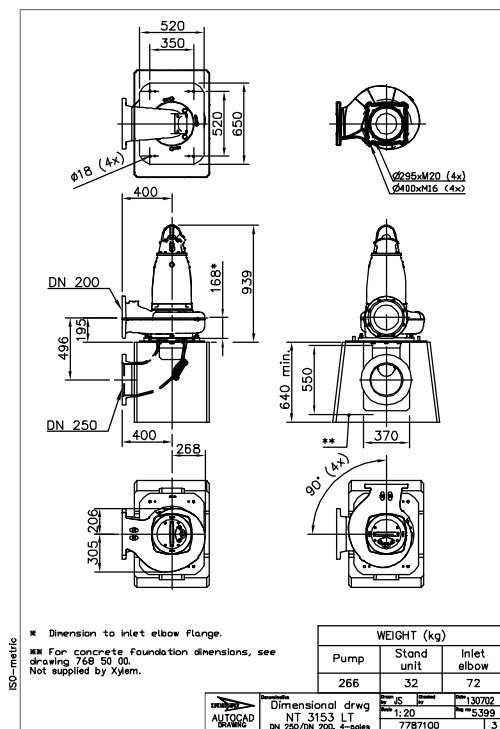
Figure 17: LT, T-installation
