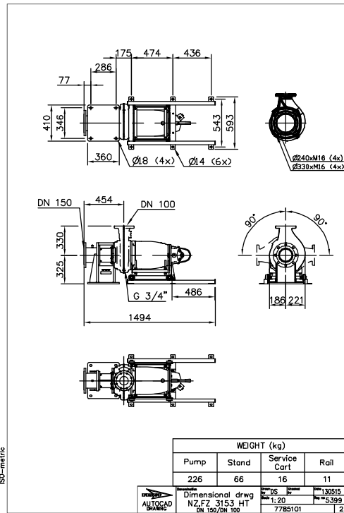
Figure 32: HT, Z-installation
