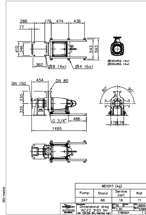
Figure 37: SH, Z-installation
