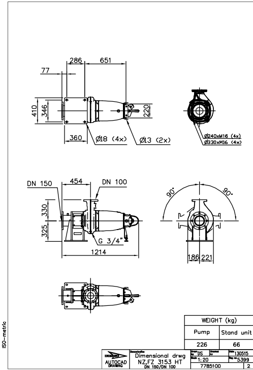
Figure 31: HT, Z-installation
