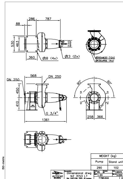
Figure 21: LT, Z-installation
