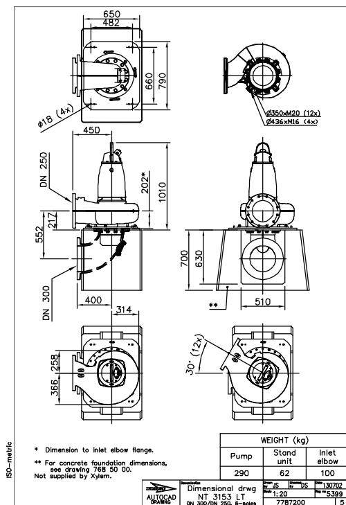
Figure 18: LT, T-installation
