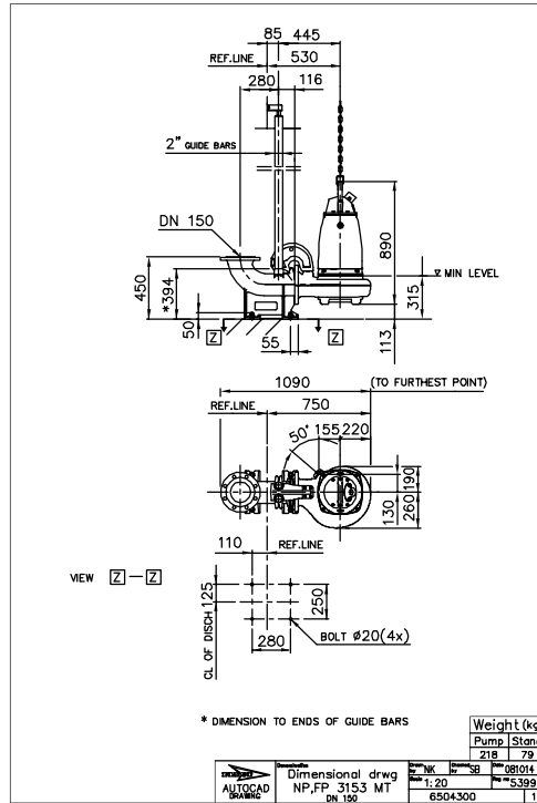
Figure 23: MT, P-installation
