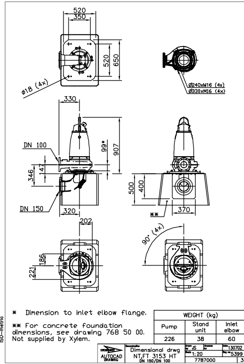
Figure 30: HT, T-installation
