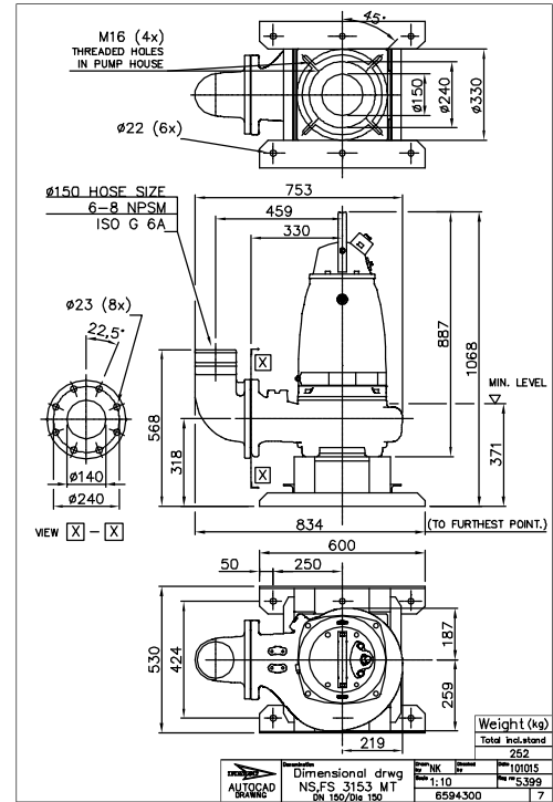
Figure 24: MT, S-installation
